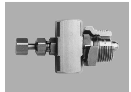
Shown is nipple XMW 0021 xx mounted on a MW nozzle.
